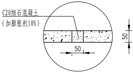
板缝B 1: 10
