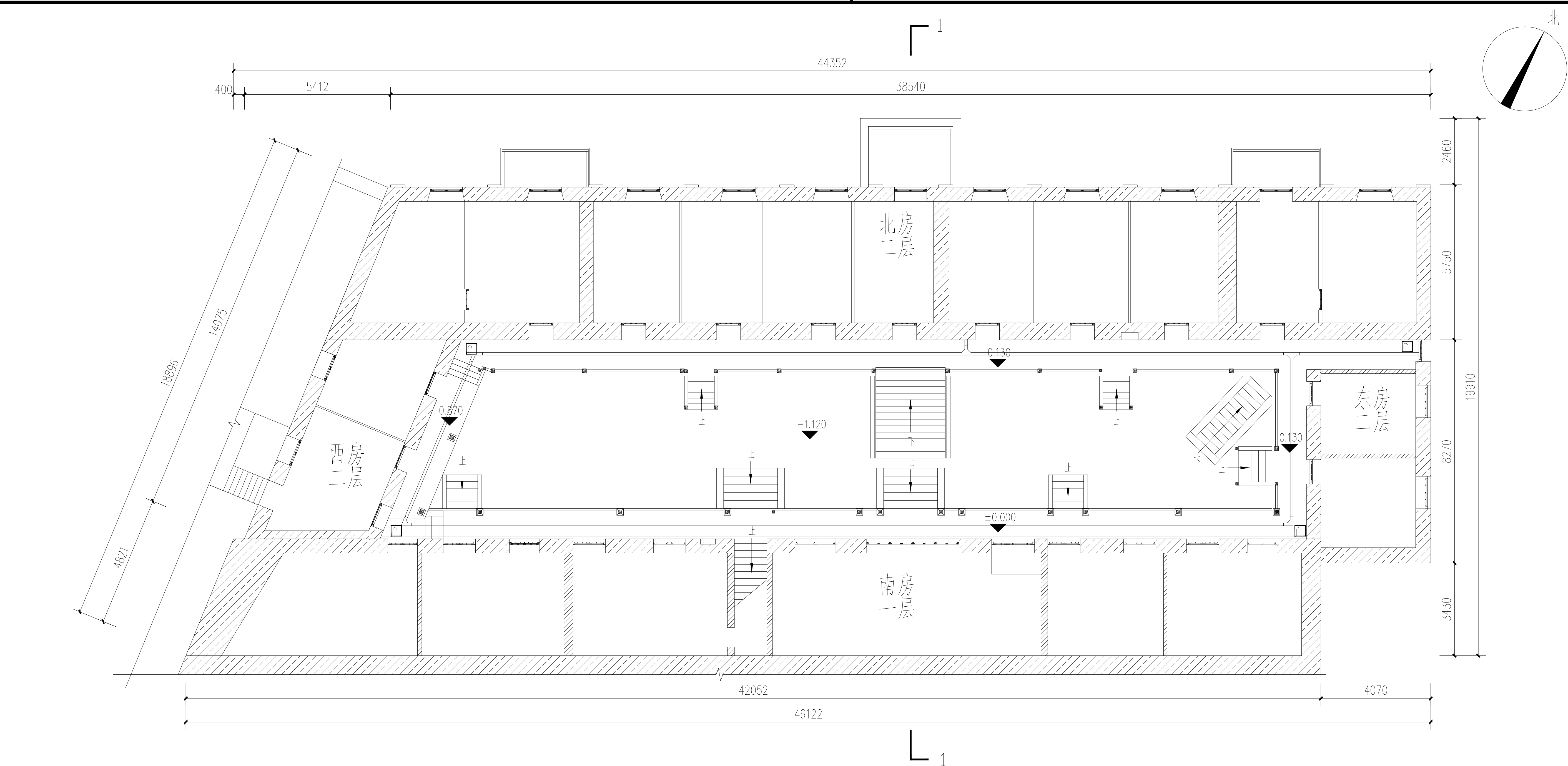
院落二层总平面图 (1:110)
