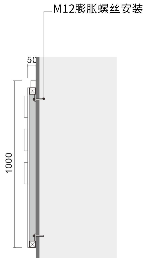
侧视图 SIDE VIEW
