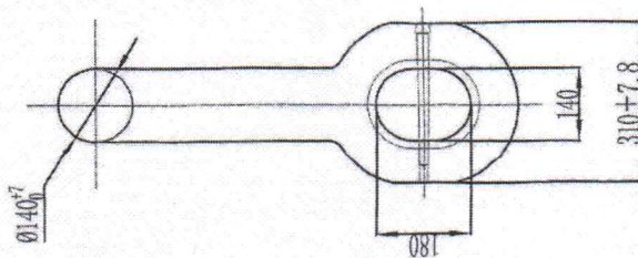
END SHACKLE (ES)
