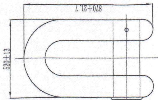
END SHACKLE (ES)
