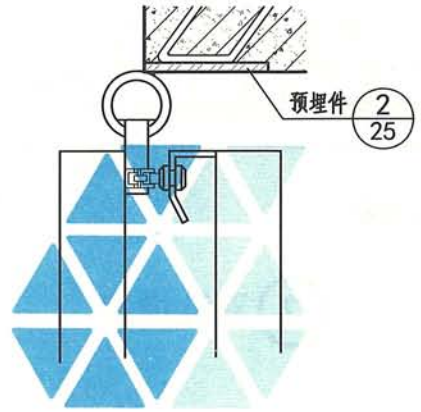
③ 门挡
