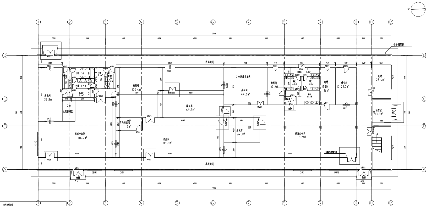
FF FIXTURE/FURNISHING PLAN 1F 平面布置图
