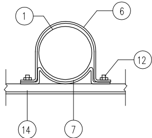
II—II
