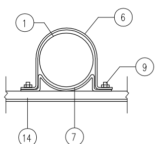
II—II
