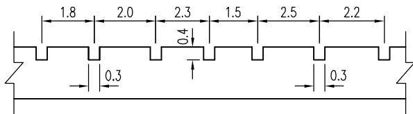
桥面及搭板面修整大样
