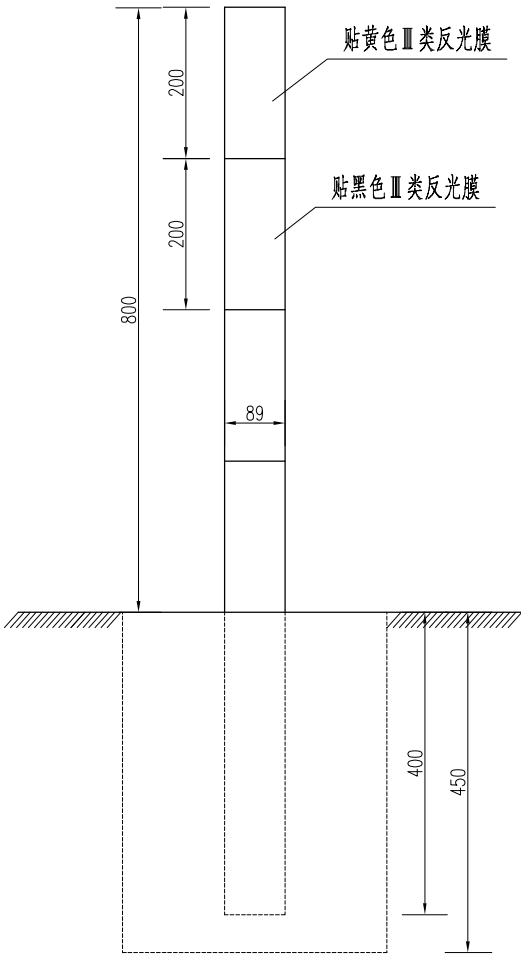
示警桩
