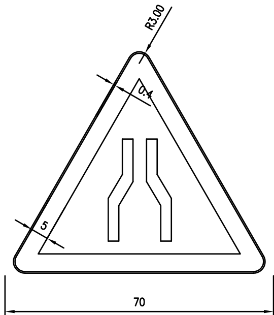
警7 (1: 10)
