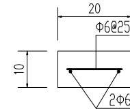
压顶配筋 1:10
