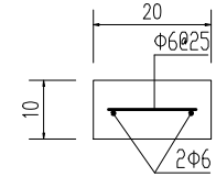
压顶配筋 1:10
