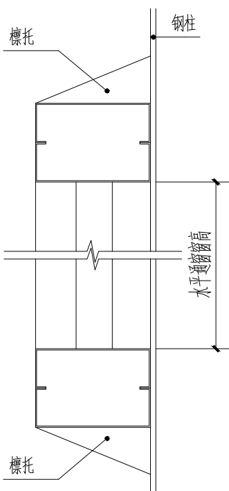
窗上下口標托布置
