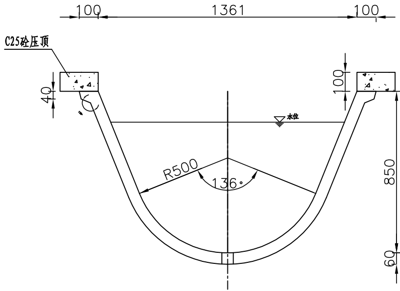
渠道衬砌横断面图 1: 20
