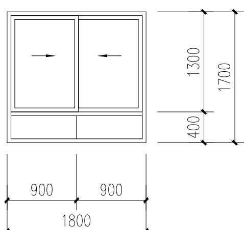
TC1817 1:50
